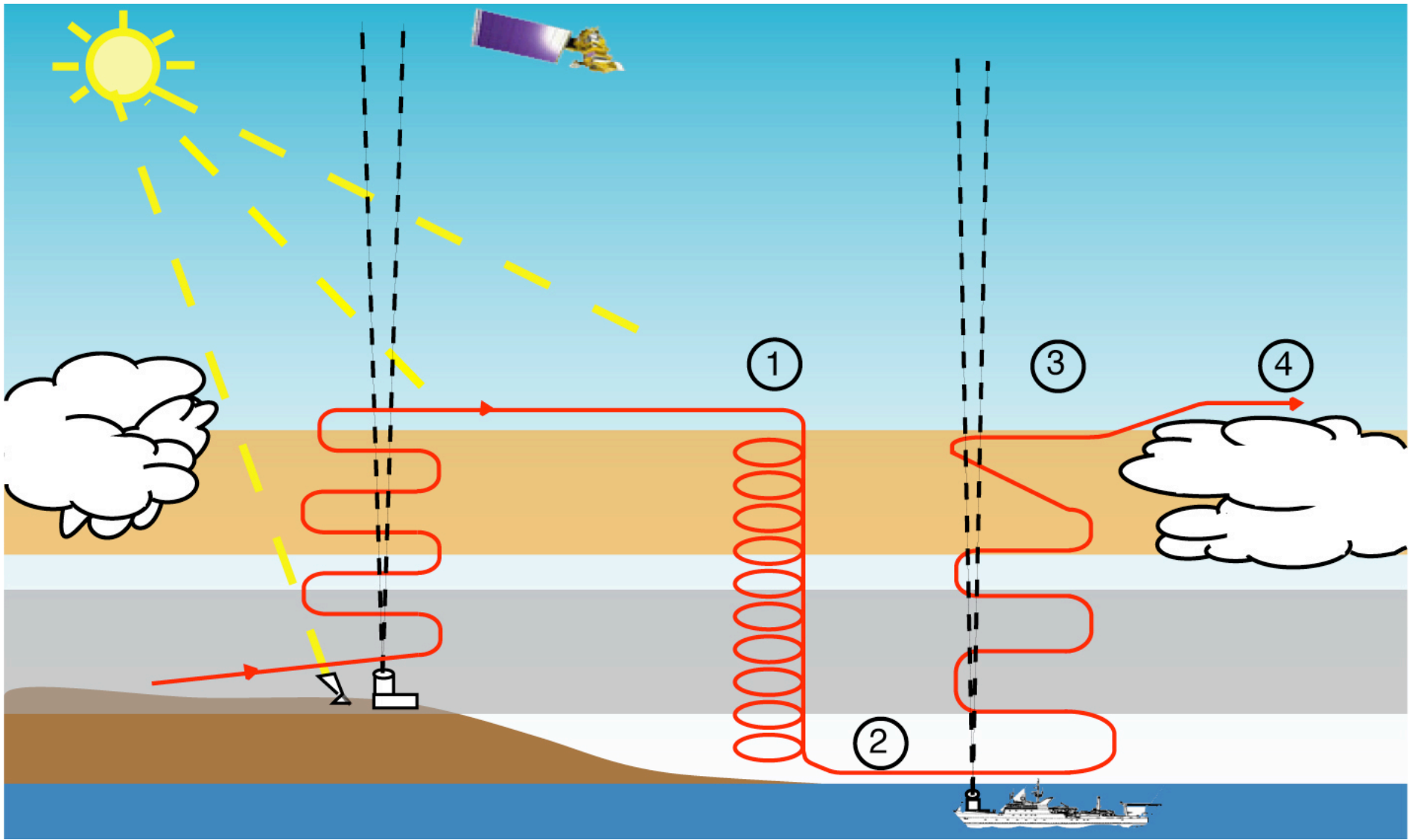
(1) Survey Vertical Profile. (2) Minimum-Altitude Transect. (3) Parking Garage. (4) Above-Cloud Transect.
