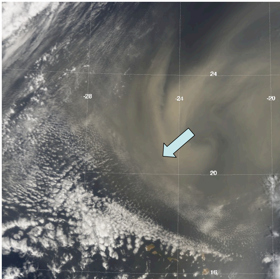
Terra MODIS 10:30 a.m.
