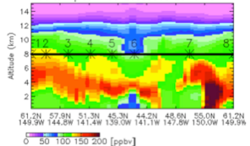
Curtain plot - CO 20060509 20-04 GMT
