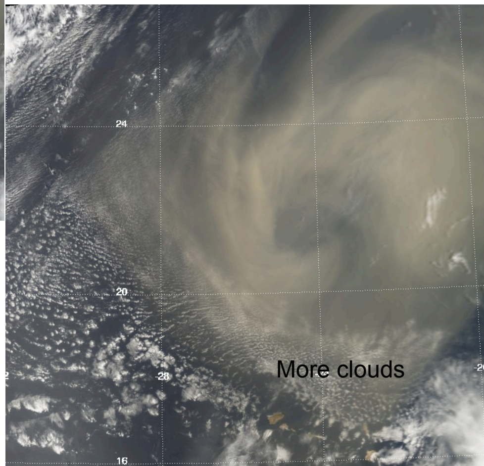
Aqua MODIS 1:30 p.m.
