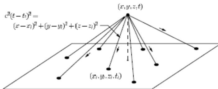
Figure 5: Basic TOA technique. Measurements of the arrival times t_i at N \geq 4 locations are used to determine the location and time of the source event (x, y, z, t) .
