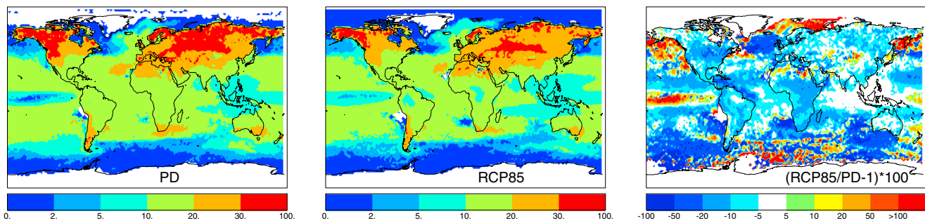
Figure 3. Cloud-to-ground percentage of total lightning for (left) PD, (middle) RCP85, and (right) the relative difference between both.
