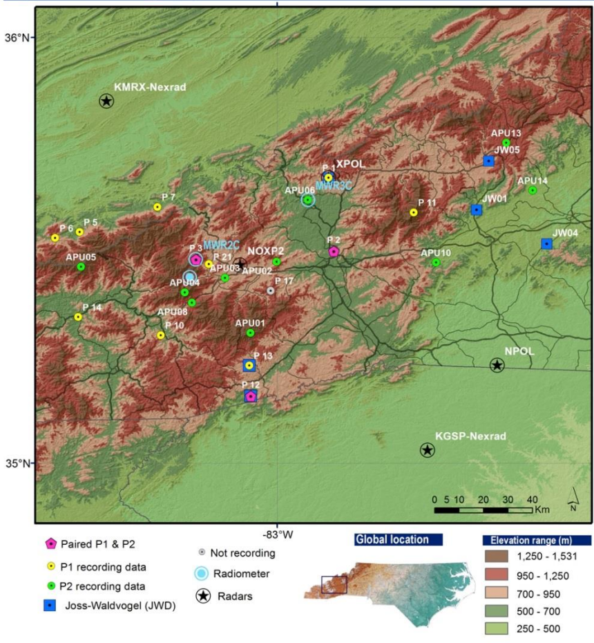
Figure 6 – Current network of fixed instrumentation during the IPHEX IOP. [This map will continue to be updated with instruments].
