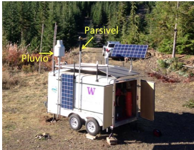
Figure 3: Instrumented trailer installed on the southern side of the Olympic Mountains. The Pluvio and Parsivel are mounted high on the trailer to keep them above the accumulating snowpack. Photo by Joe Zagrodnik. [image source: https://earthobservatory.nasa.gov/blogs/fromthefield/category/olympex-2015/ ]
